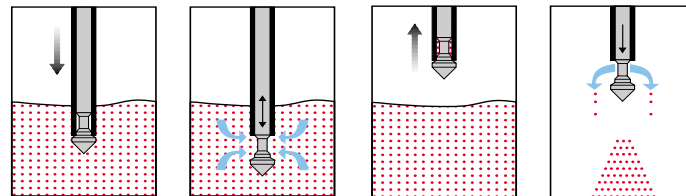
1. Pushing in lance 2. Opening head 3. Close head, pull back lance 4. Emptying MicroSampler
