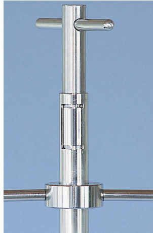
Double-sample possible without moving the lance in the bulk material
