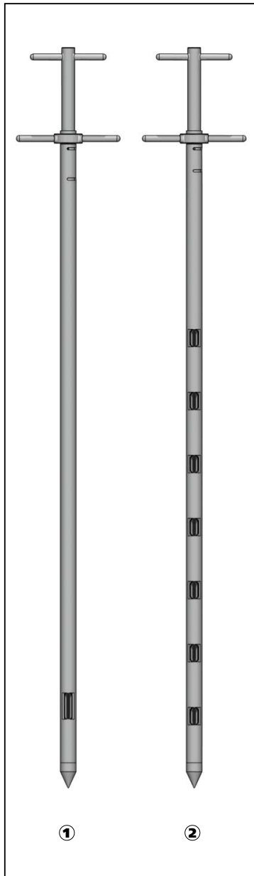
Double-sample possible without moving the lance in the bulk material
